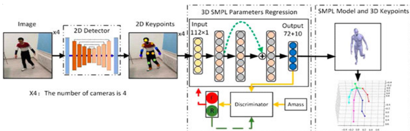
Figure 1 Pose estimation
